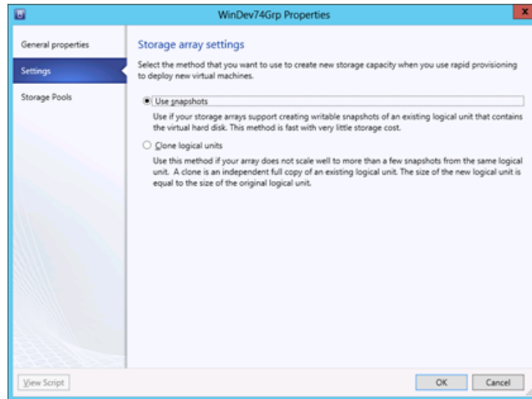
Figure 13: Storage Array Settings
