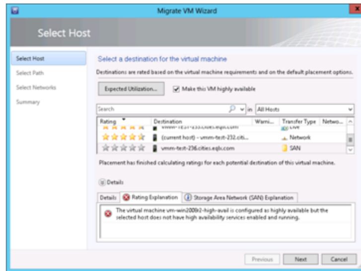
Figure 21: Rating Explanation Tab
