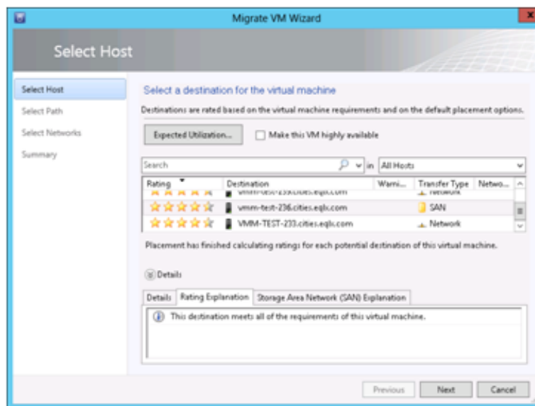
Figure 20: Migrate VM Wizard—Select Host Screen
