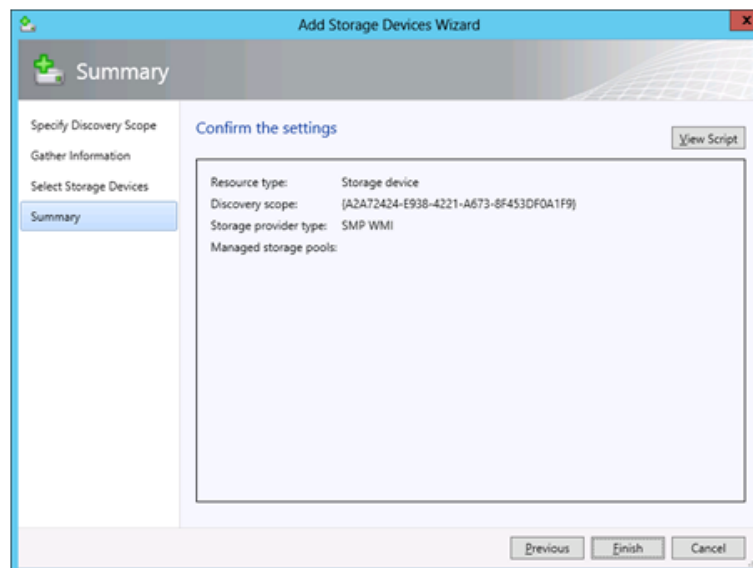
Figure 8: Summary Screen
