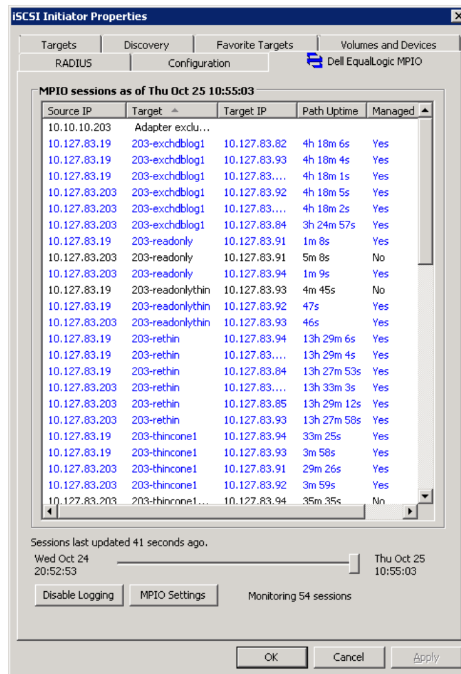
Figure 4: MPIO Properties Tab in the iSCSI Initiator
