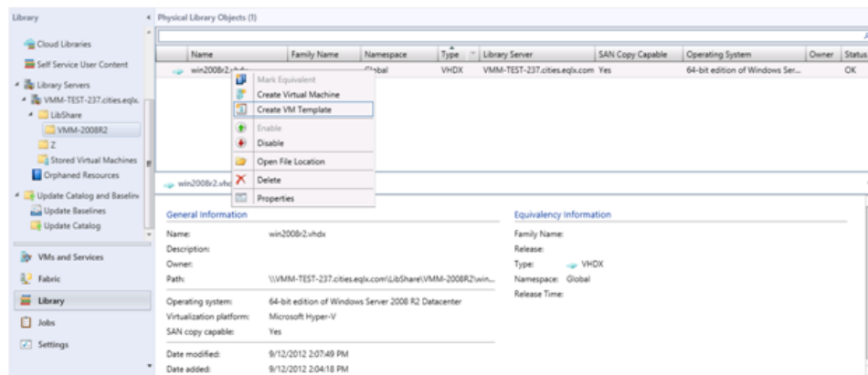
Figure 16: Create VM Template Screen
