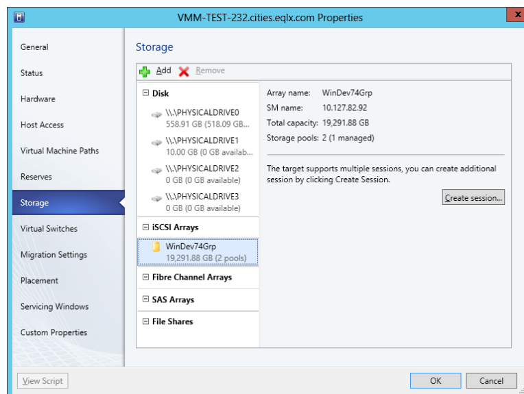
Figure 10: Storage iSCSI Arrays Screen
